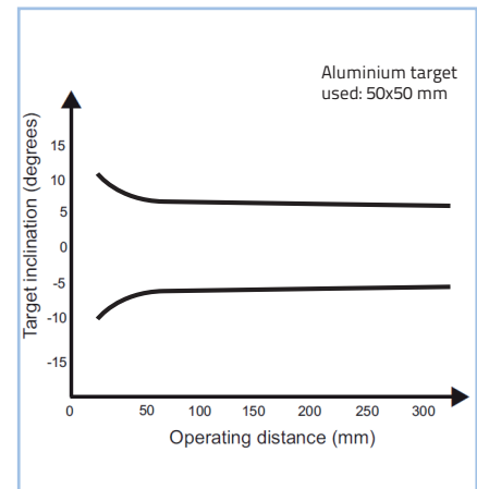
Maximum target inclination (models with analog output)
