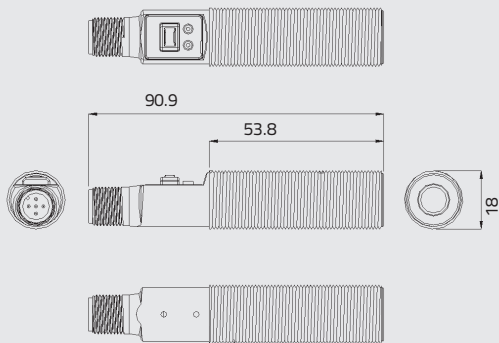
AXIAL VERSION - US18 PA-5-N03-XX
