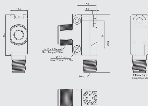
M18 Right Angle US18 PL-5-N03-NH/PH
