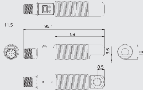
RADIAL VERSION - US18 PR-5-N03-XX
