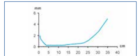
Resolution - axial
