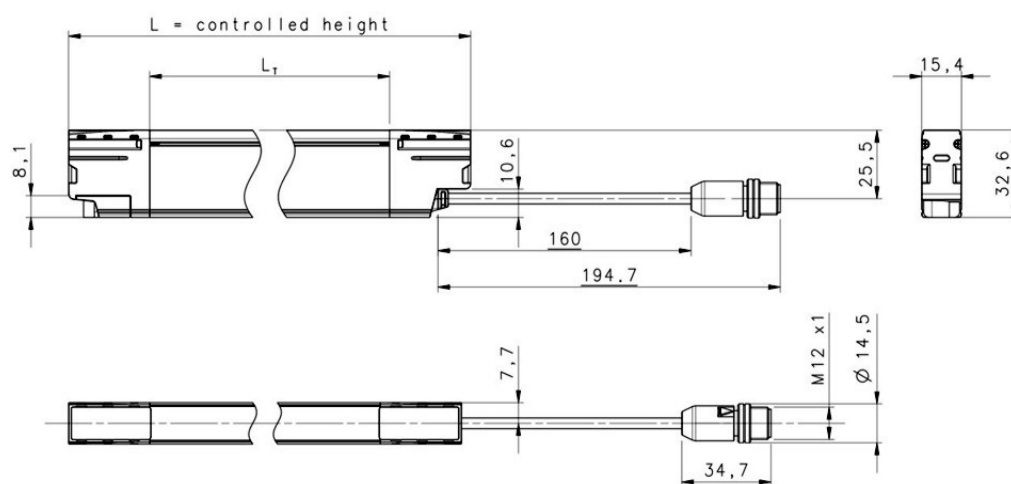
Figure 1 - Overall dimensions (mm)
