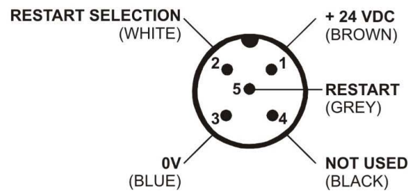
Figure 2 - Emitter
