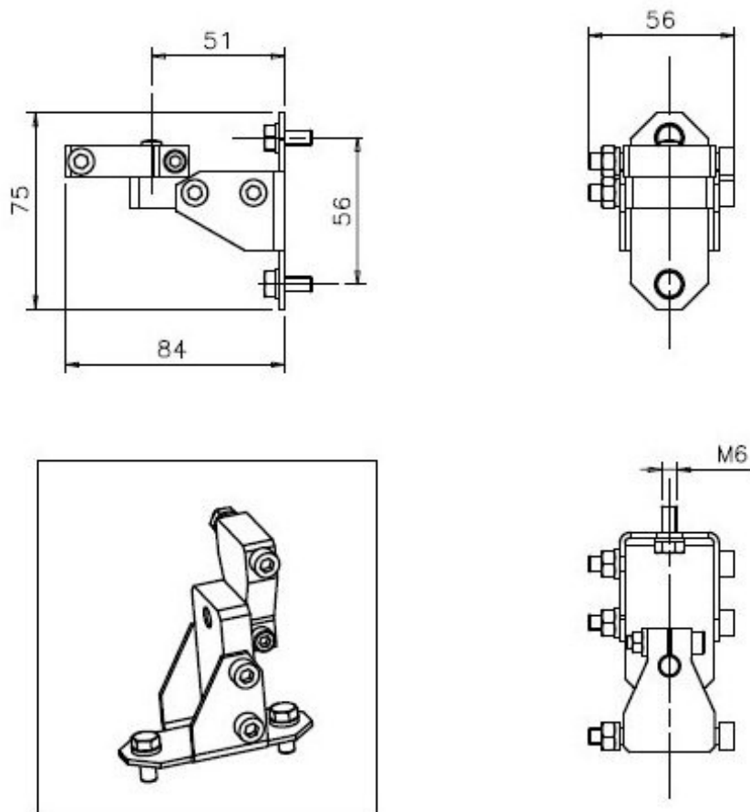
Figure 8 - Mounting kit
