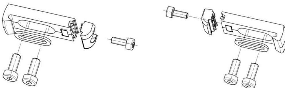
Figure 1 - “C” type brackets kit
