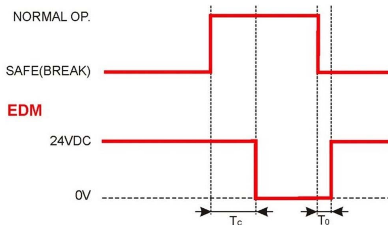
Figure 6 - EDM timings
