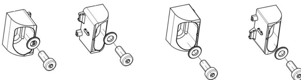
Figure 2 - “O” type brackets kit
