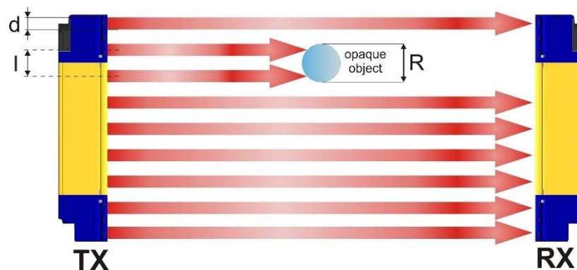
Figure 1 - Detection capability
