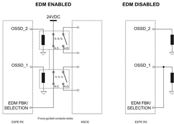
Figure 4 - EDM connection
