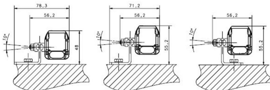
Fig 81 - Angled fixing bracket + Orientable support
