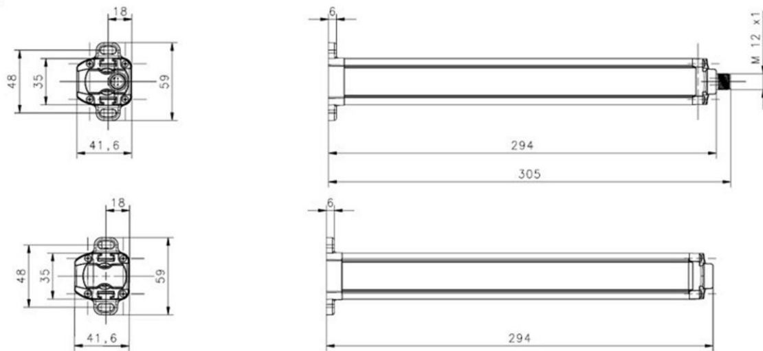
Fig 109 - Dimensions (mm)
