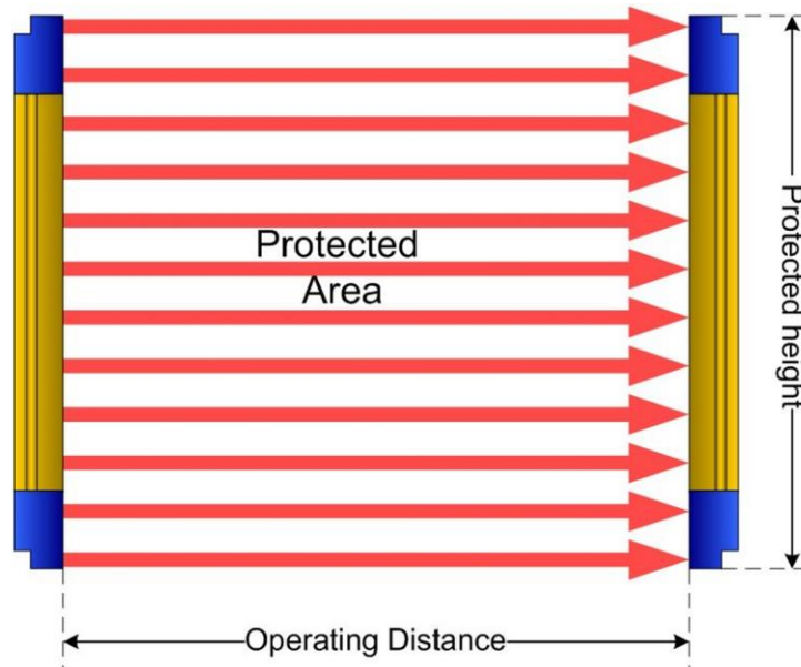
Fig 3 - Detection Zone
