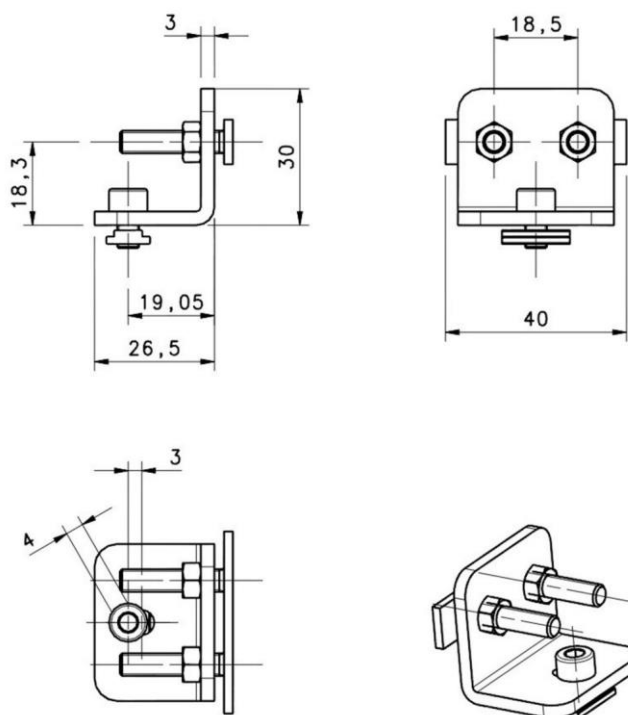
Fig 90 - Fixing kit
