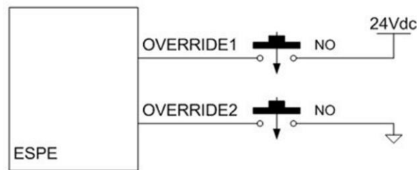
Fig 66 - Override connection
