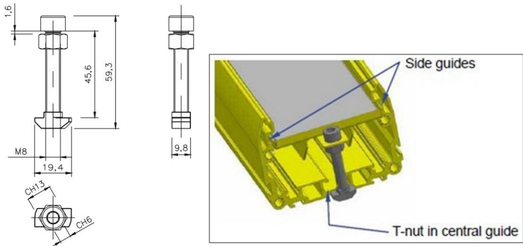
Fig 97 - Mounting kit
