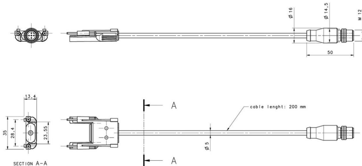
Fig 98 - TX - Pigtail cable
