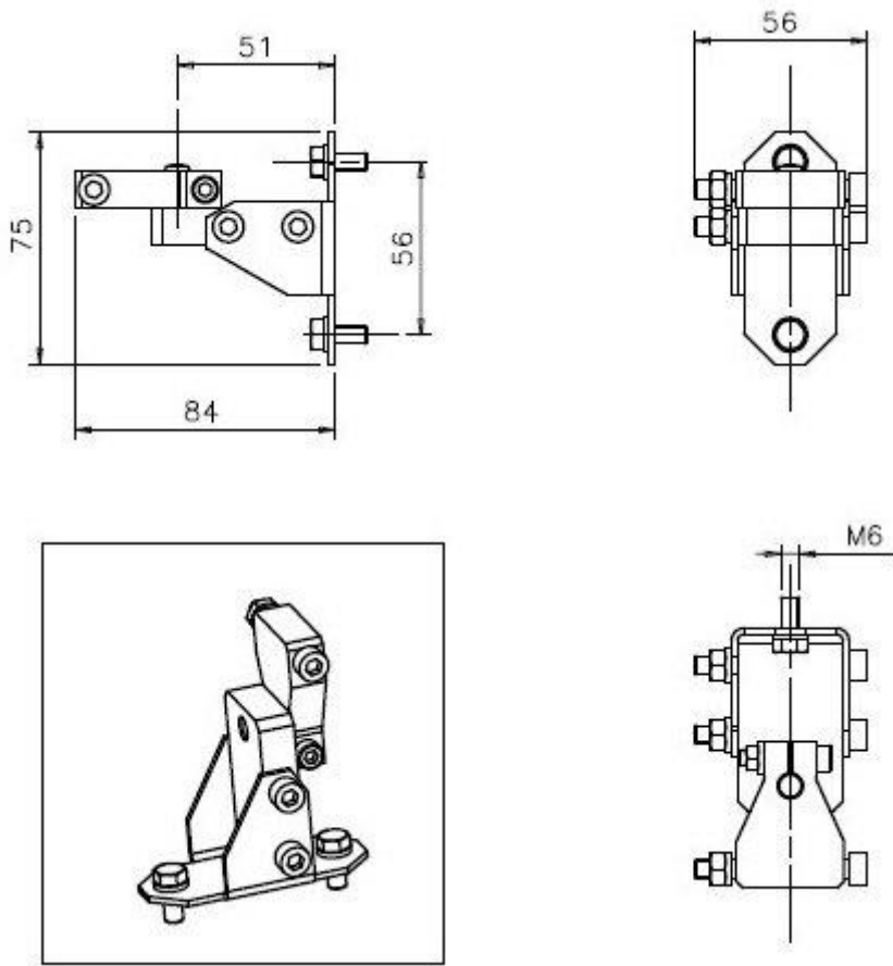
Fig 96 - Mounting kit
