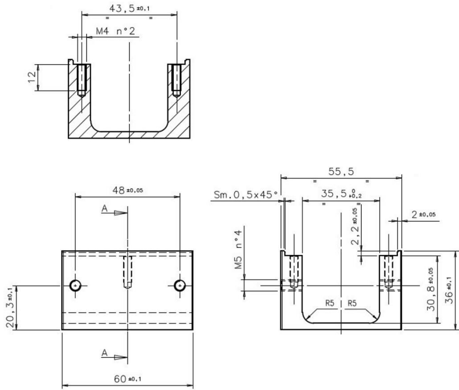
Fig 110 - Mounting bracket
