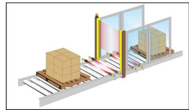
Fig 56 - Linear version with external Muting sensors
