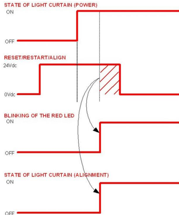
Fig 35 - Alignment timings
