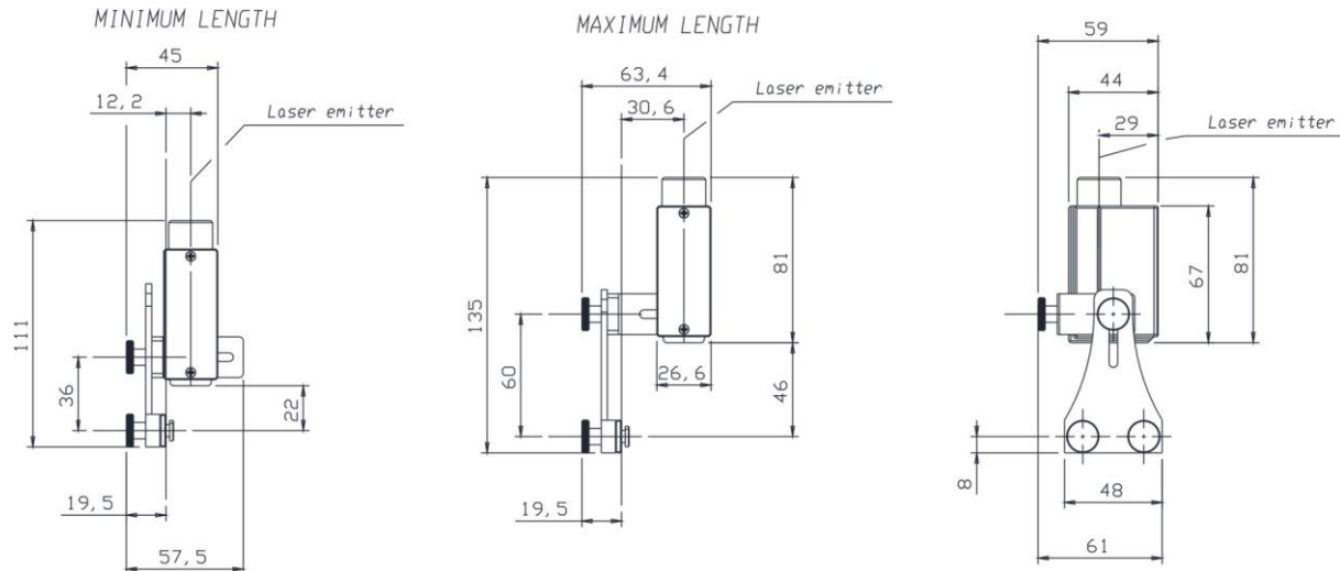
Fig 100 - Dimensions (mm)
