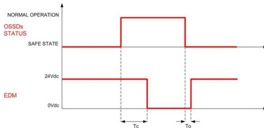
Fig 49 - EDM timings (PNP configuration)
