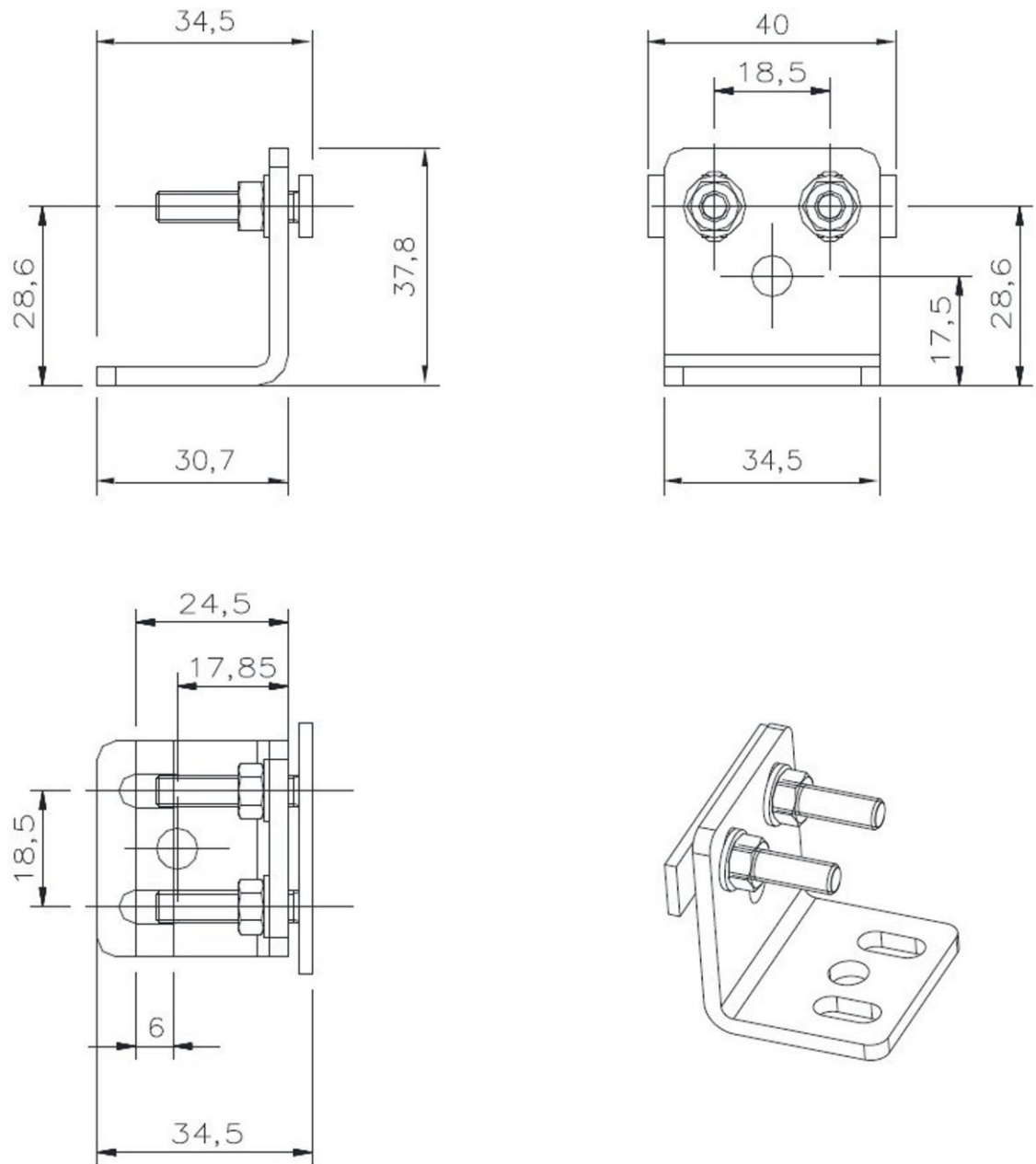
Fig 76 - Dimensions (mm)
