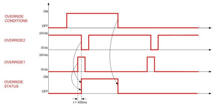
Fig 69 - Override timings (edge trigger)
