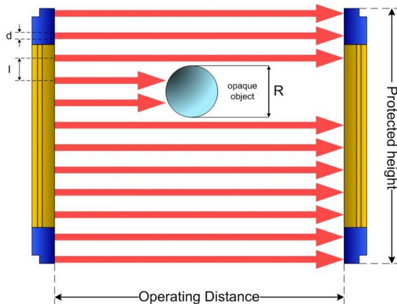
Fig 2 - Detection capability
