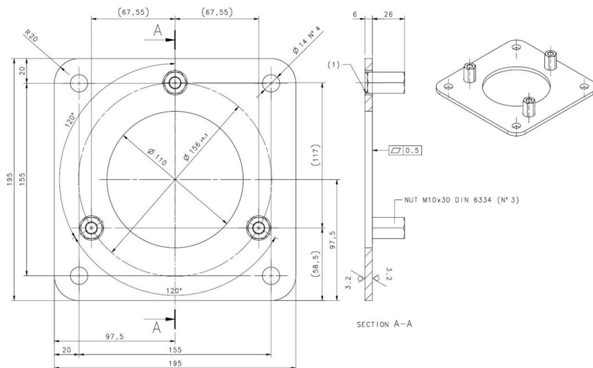
Fig 91 - Dimensions (mm)
