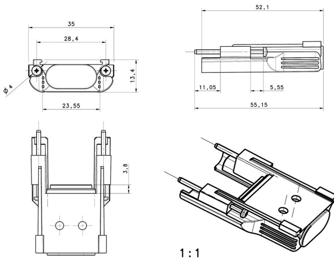
Fig 77 - Dimensions (mm)
